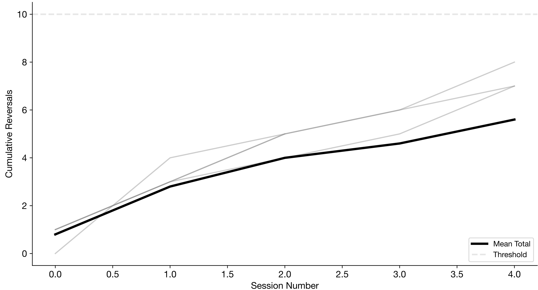
Cumulative Total Reversals Over Time (n=5 subjects; sessions per subject=1–5)
